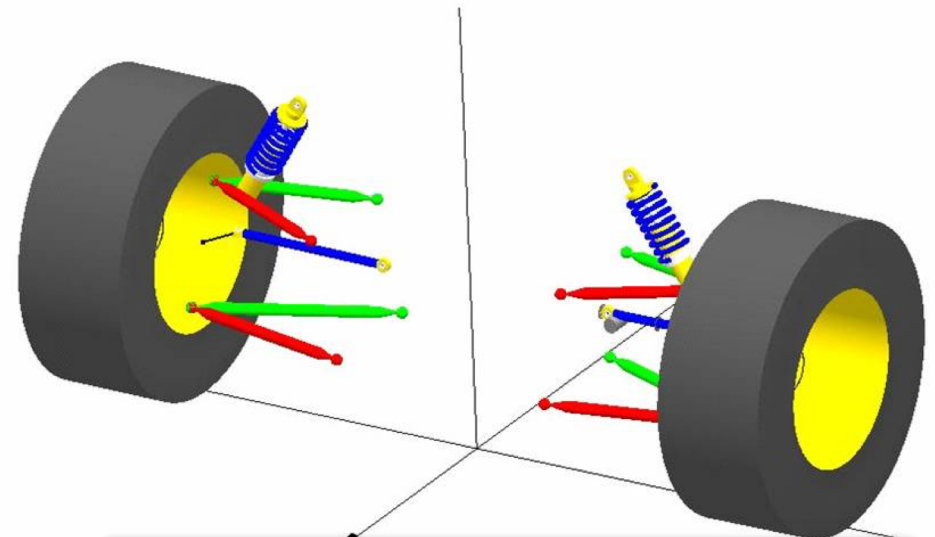
Digitally Analysed Suspension
